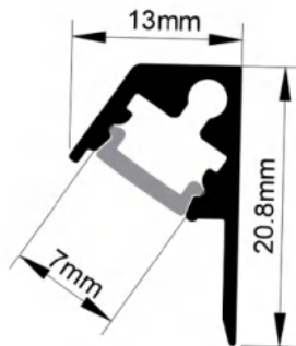
Dimension
