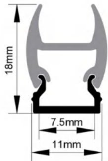
Dimension
