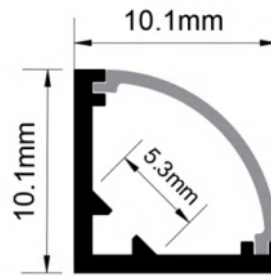
Dimension
