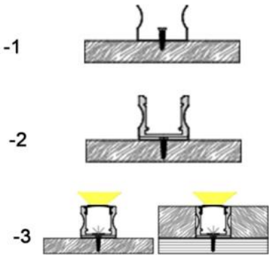
Installation steps
