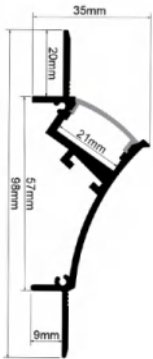
Dimension
