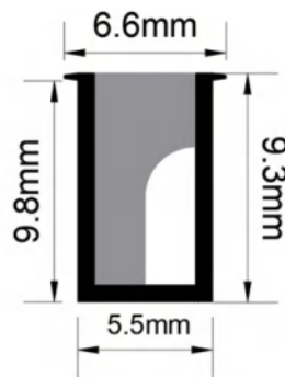
Dimension
