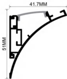
Dimension
