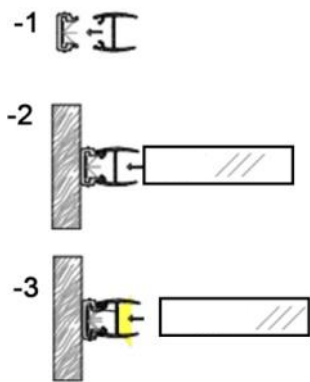
Installation steps
