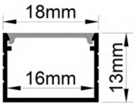
Dimension
