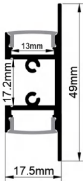
Dimension
