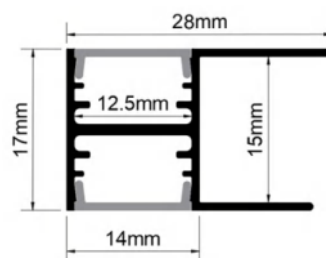
Dimension
