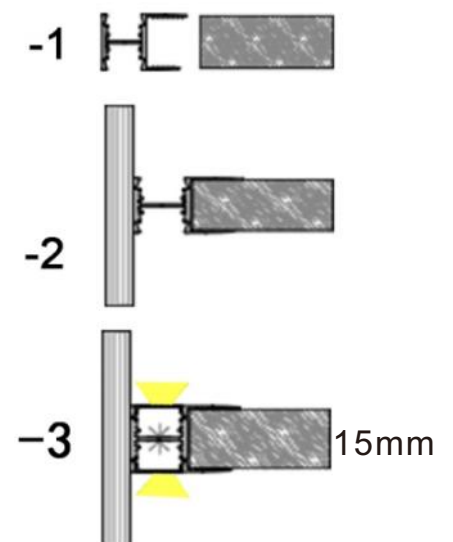
Installation steps
