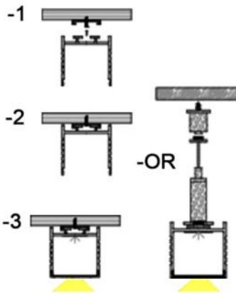
Installation steps
