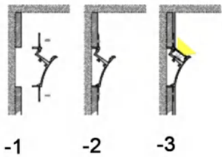
Installation steps
