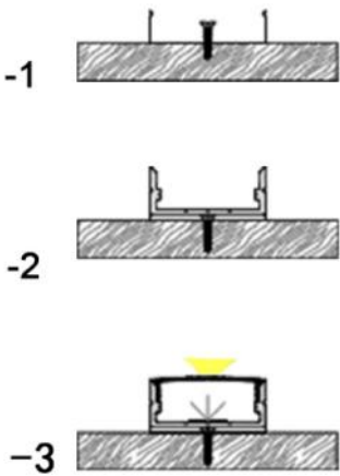
Installation steps
