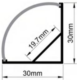
Dimension
