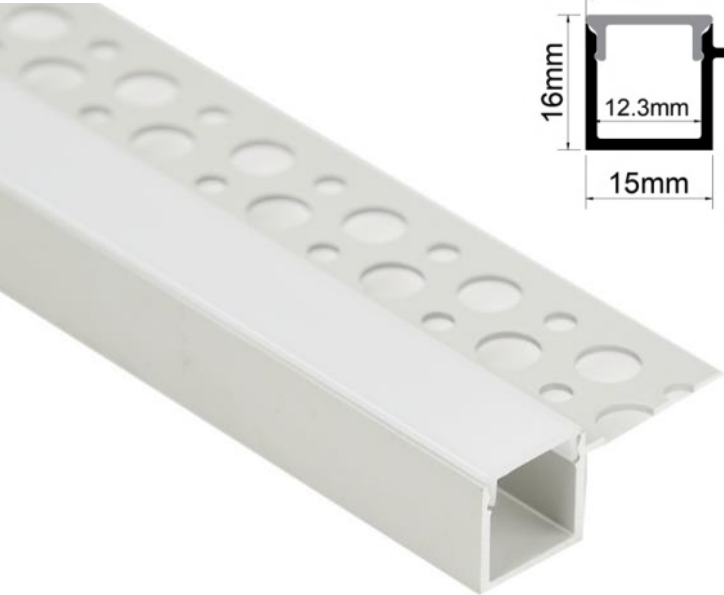
Dimension
