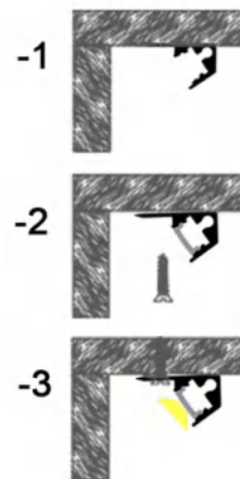
Installation steps
