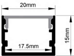
Dimension
