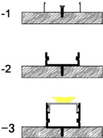
Installation steps
