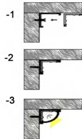
Accessories
