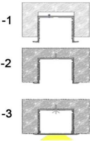
Installation steps
