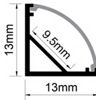
Dimension
