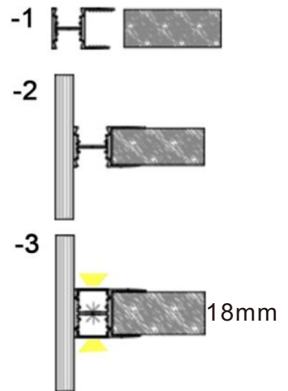
Installation steps
